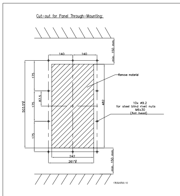
Illustration 1.2: B1 Enclosure
