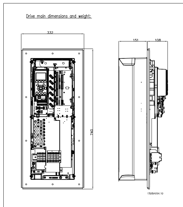
Illustration 1.14: B2 Enclosure
