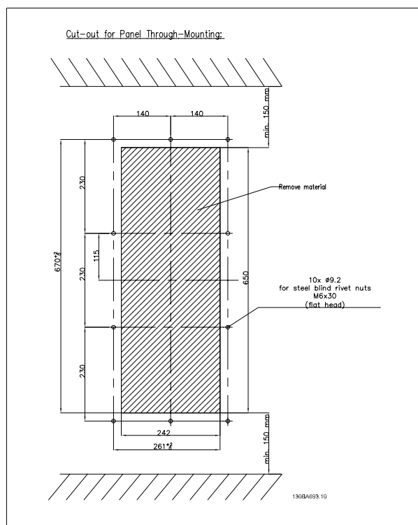
Illustration 1.3: B2 Enclosure
