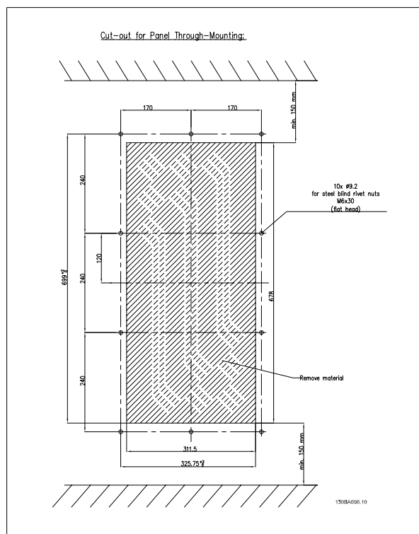
Illustration 1.4: C1 Enclosure
