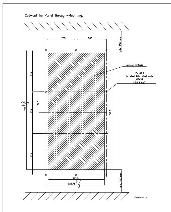
Illustration 1.5: C2 Enclosure
