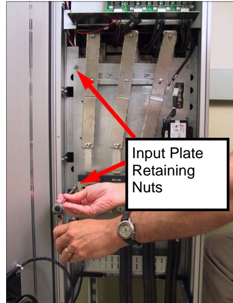
Photo 5. Removing Input Plate Retaining Nuts
