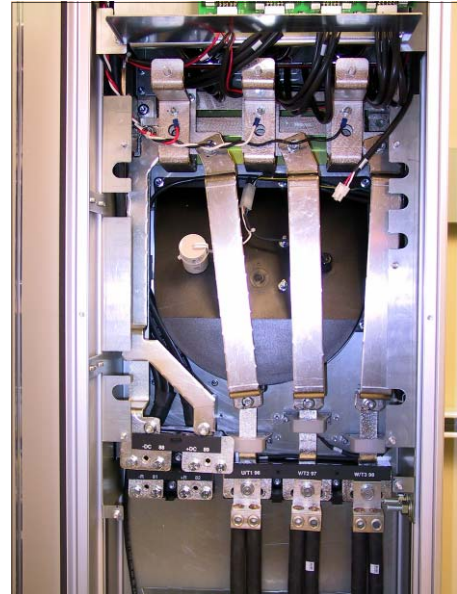
Photo 7. VLT Frame D2 with Input plate removed
