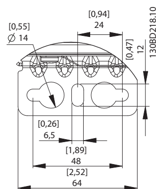
Illustration 9.31 Mounting Hole
