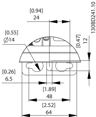
Illustration 9.3 Mounting Hole
