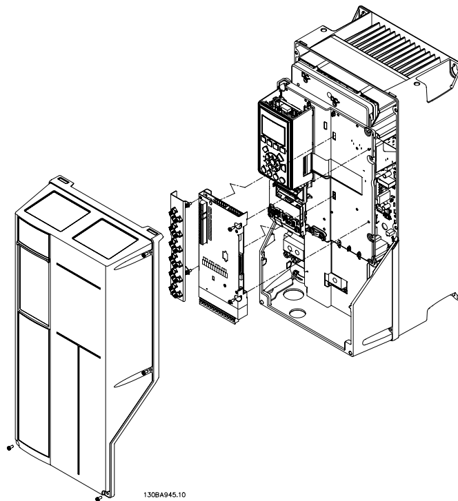
Illustration 1.4: Enclosures B (except B3) and C.
