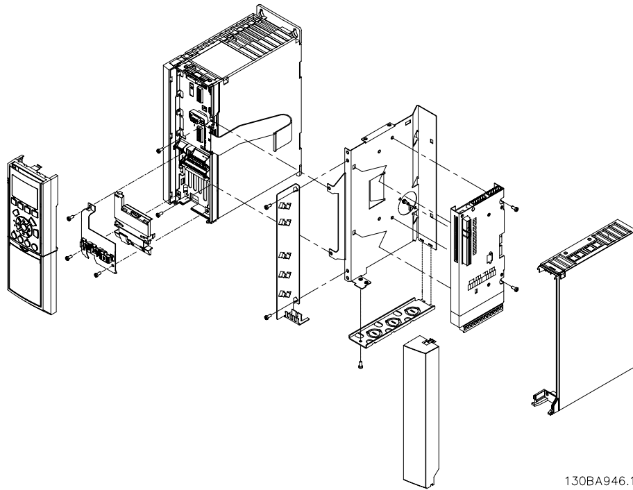
Illustration 1.3: Enclosure A2, A3 (and B3) 40 mm (only one C option).
