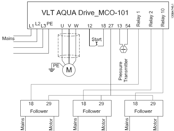
Illustration 1.16: Electrical wiring. Terminal 27 on master drive is used as pulse output reference. Terminal 29 on the follower drives is used as pulse input reference. All follower drives are connected to mains and motor the same way as the master drive symbolized with the text: Mains and Motor .
