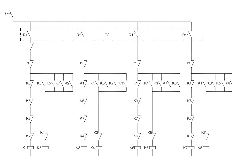
Illustration 1.5: Control circuit alternating lead pump (4 pumps).
