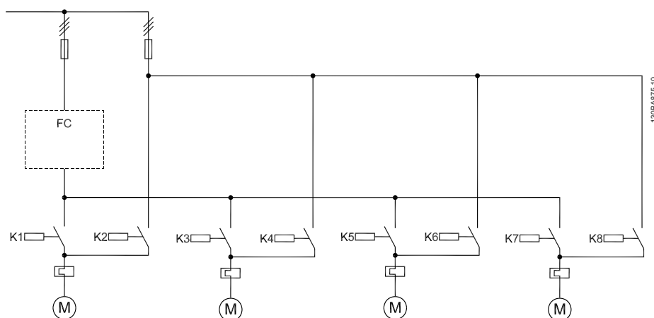
Illustration 1.6: Mains circuit alternating lead pump (4 pumps).
