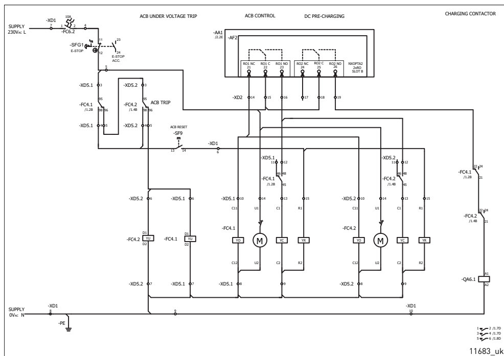
Figure 101. Wiring diagram for controls, OPTA2
