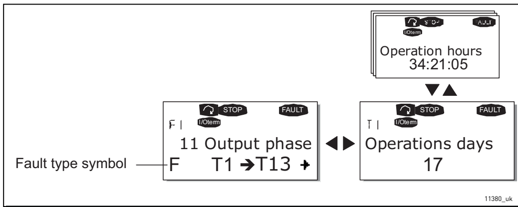
Figure 66. Fault display
