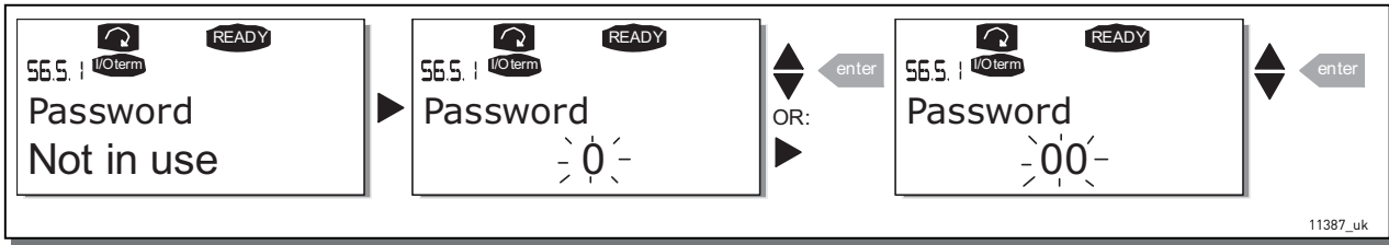
Figure 73. Password setting
