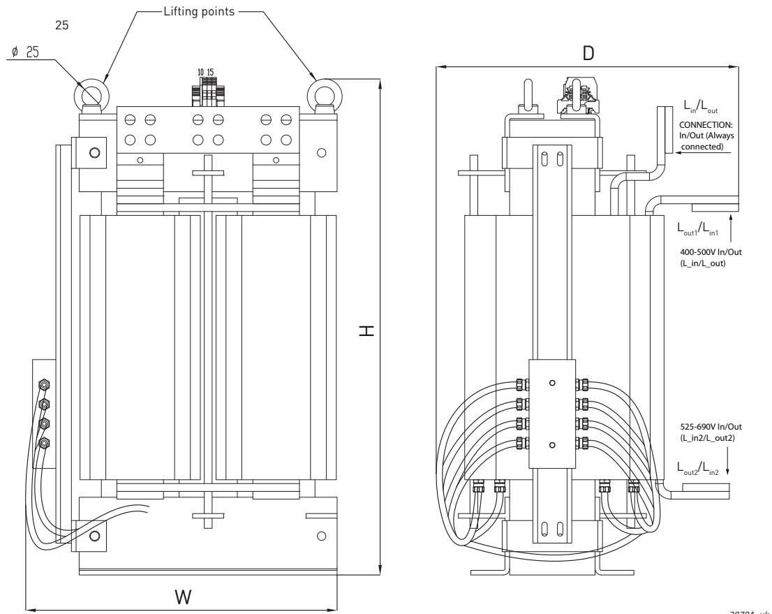
Figure 89. Example of L_{afe} choke of a VACON ® RLC filter
