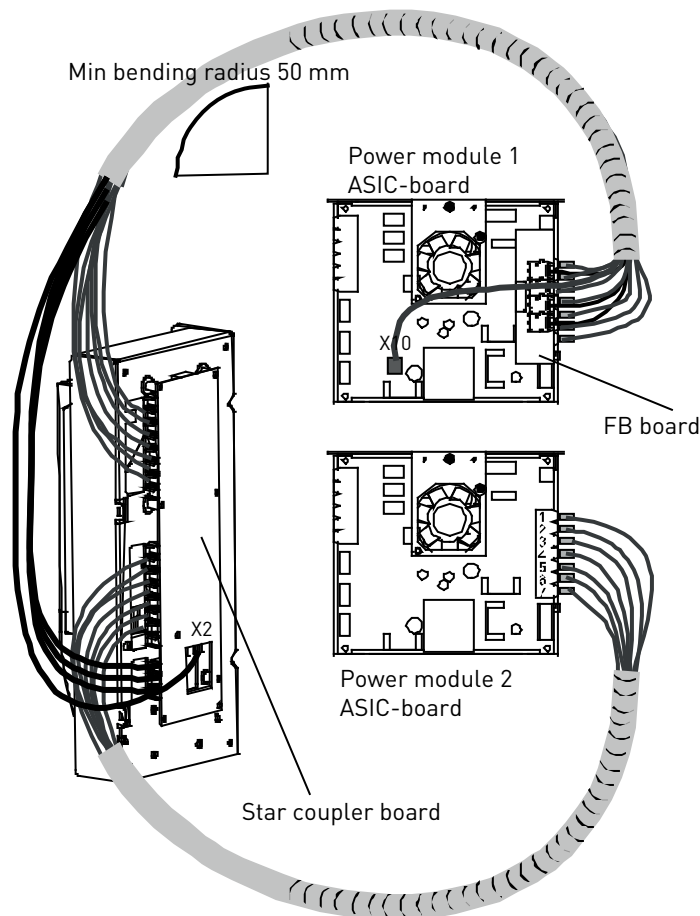
Figure 58. Connecting the power supply and control cables to the control unit, 2xCh64 and 2xCH74
