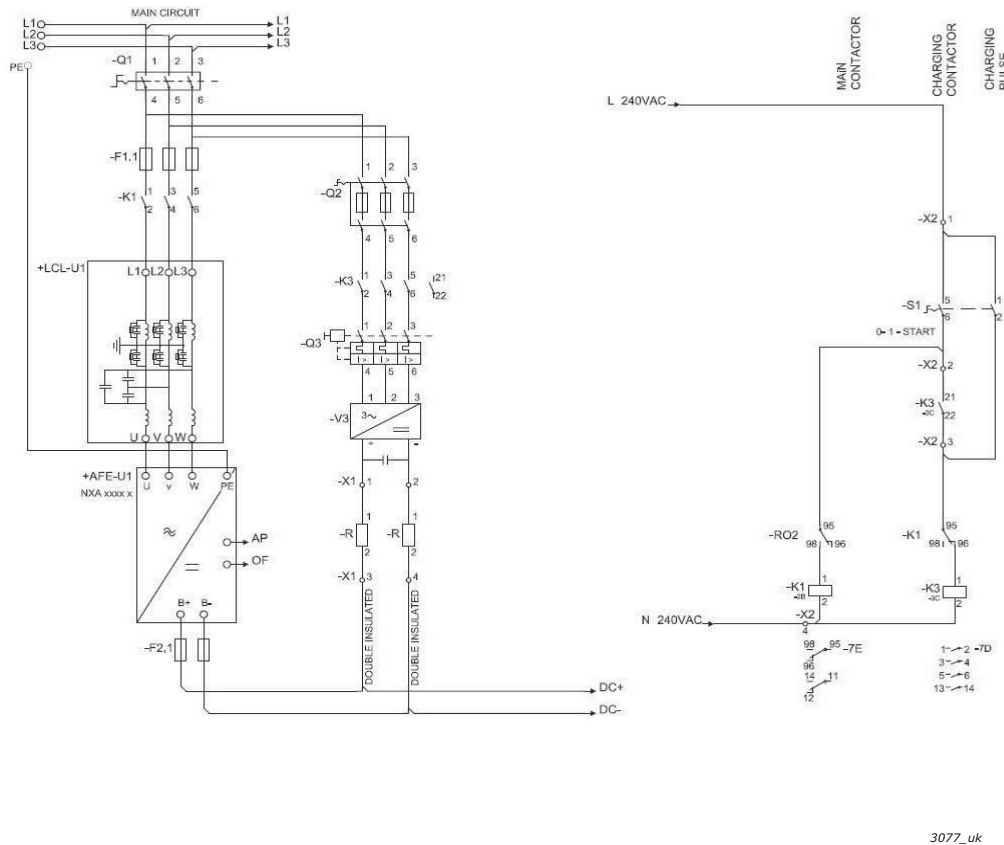
Figure 94. Wiring diagram for AFE unit
