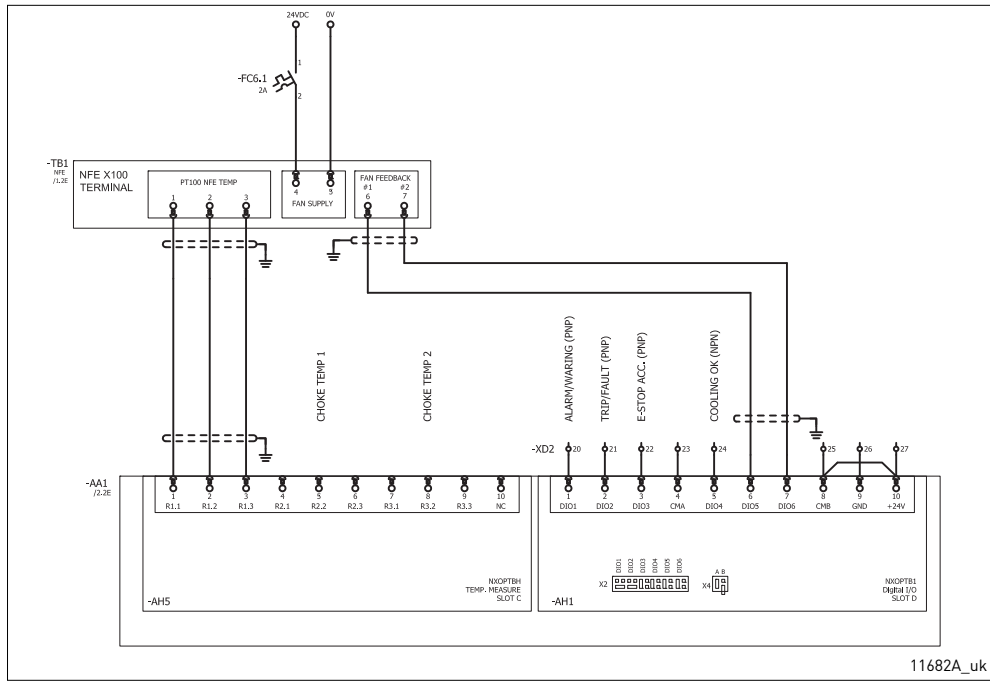
Figure 100. Wiring diagram for controls, OPTBH, OPTB1
