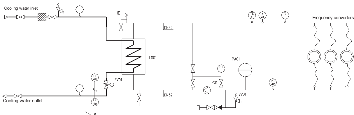
Figure 25. Example: PI-diagram of the cooling system and the connections
