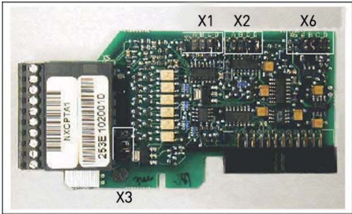
Figure 48. Jumper blocks on OPT-A1
