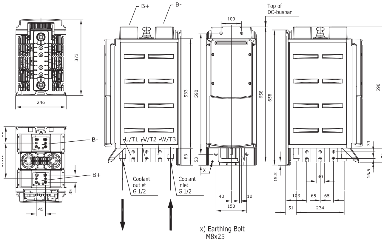
Figure 12. VACON® Liquid-Cooled inverter, CH61
