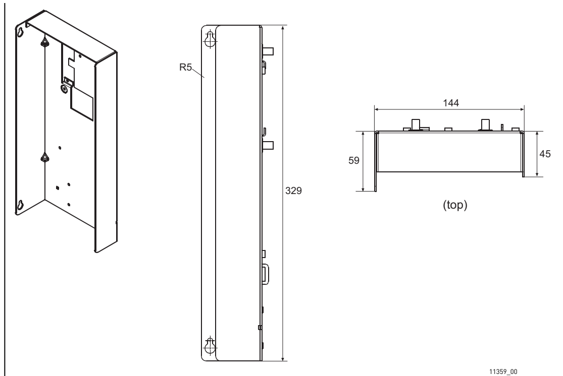
Figure 50. Control unit mounting box dimensions
