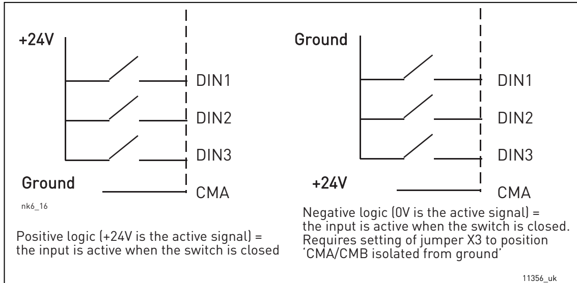
Figure 47. Positive/Negative logic
