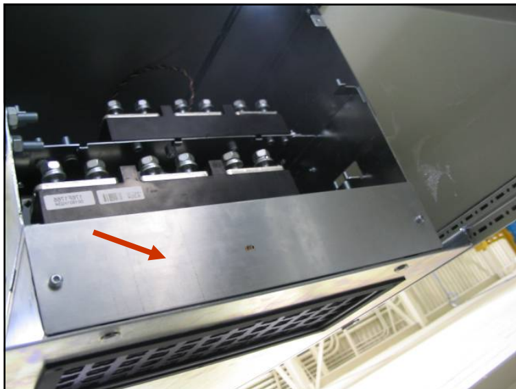
Figure 14. Bottom air inlet cover installed
