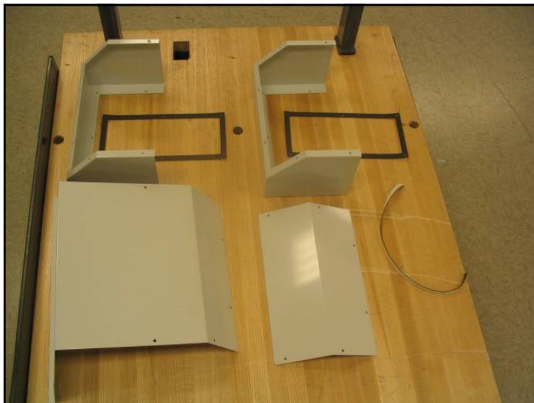
Figure 1. Air deflector components
