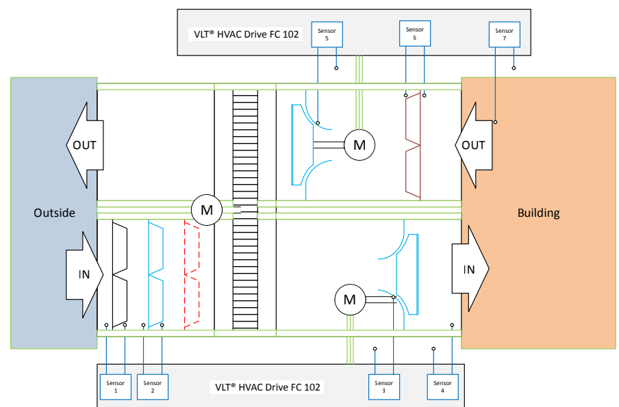
Example of installation: This air handling unit is equipped with 7 sensors. The inlet and outlet are controlled by separate VLT® HVAC Drives. Additional filters are optional.
